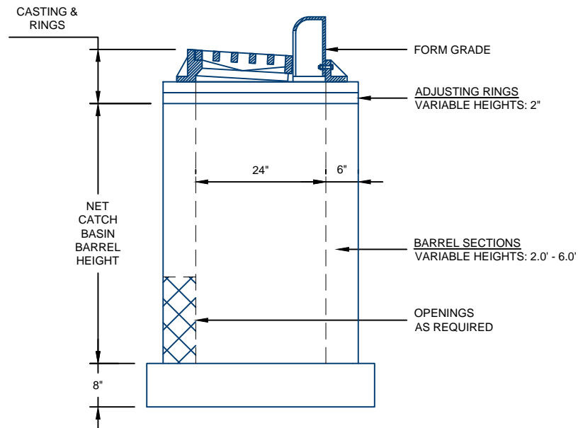
ELEVATION VIEW
