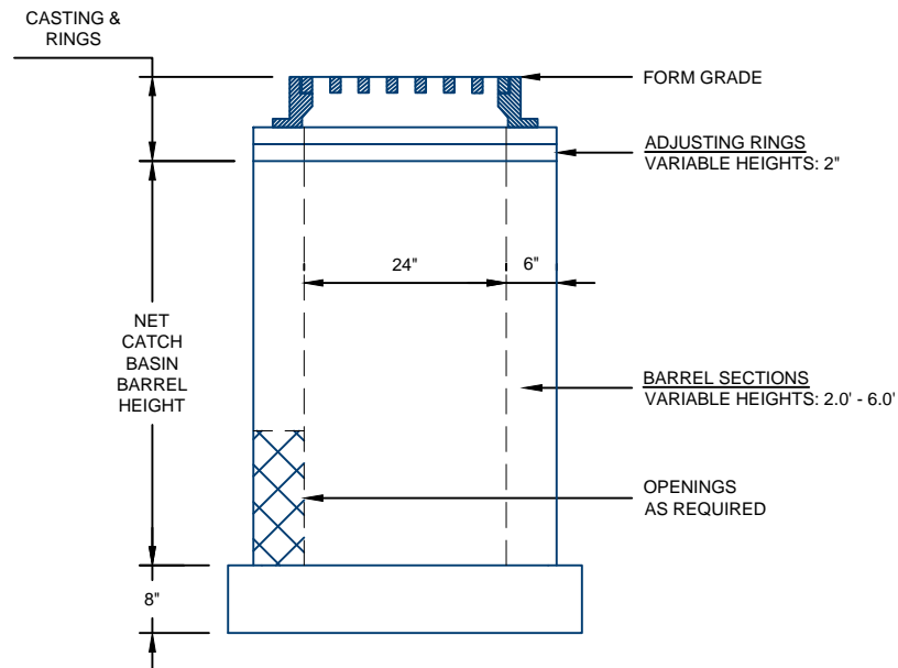
ELEVATION VIEW
